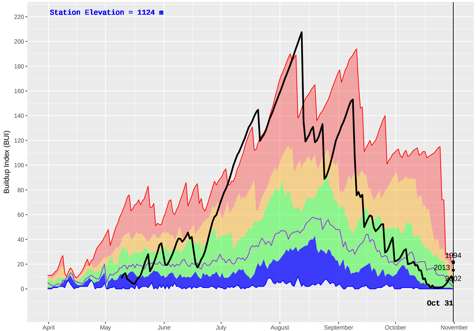
COLDSCAUR LAKE (232) : Historical (1979–2016) and Current (2017) Noon Buildup Index (BUI)
