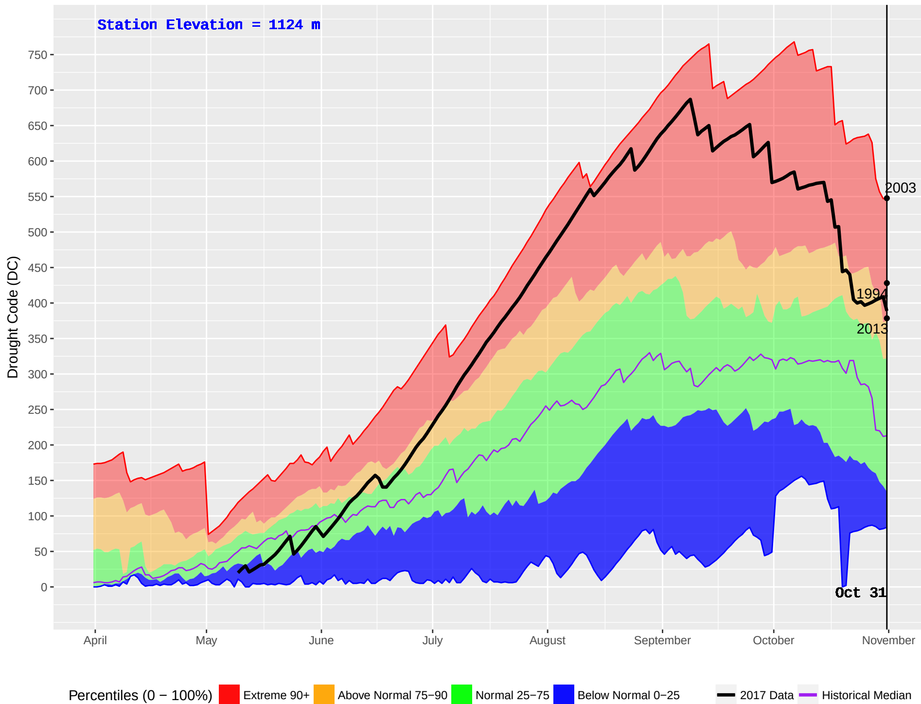
COLDSCAUR LAKE (232) : Historical (1979–2016) and Current (2017) Noon Drought Code (DC)
