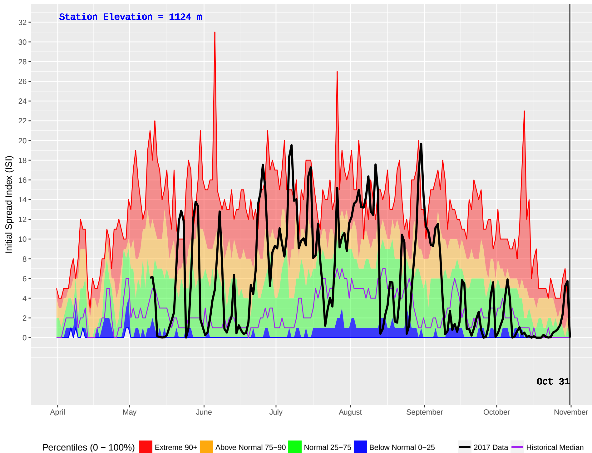
COLDSCAUR LAKE (232) : Historical (1979–2016) and Current (2017) Noon Initial Spread Index (ISI)
